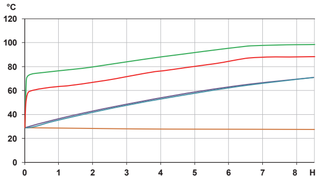
Variation in the temperature versus time of a 220-liter metal drum, filled with water, heated by a silicone heating belt 200mm wide, without thermal insulation, power 1500W (surface load 0.5W/cm²).
